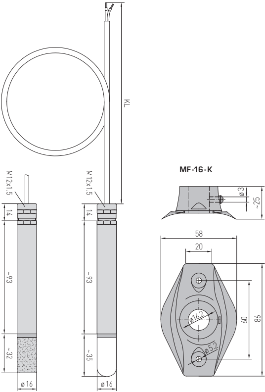
Dimensional drawing
