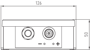
Dimensional drawing
